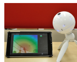
Sound source probing and visualization system
