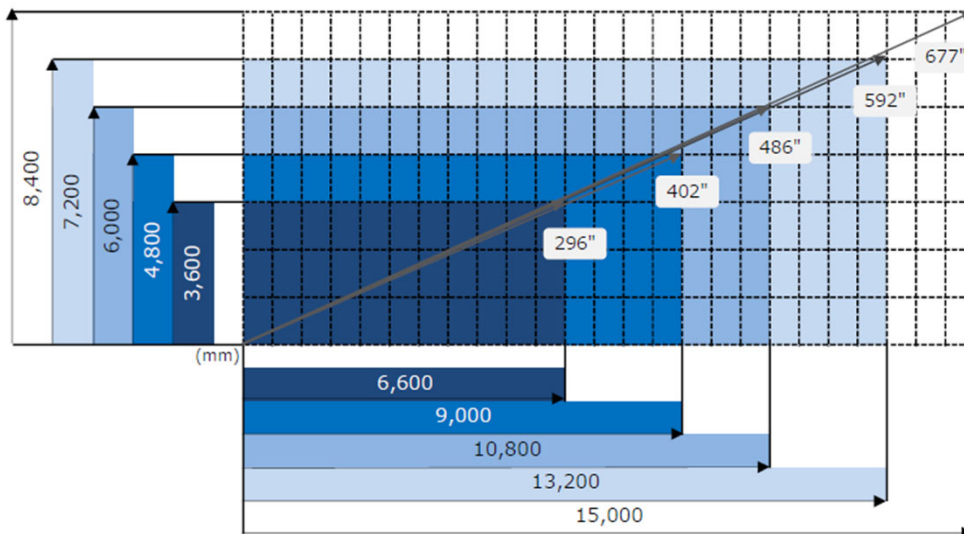
Configuration chart
